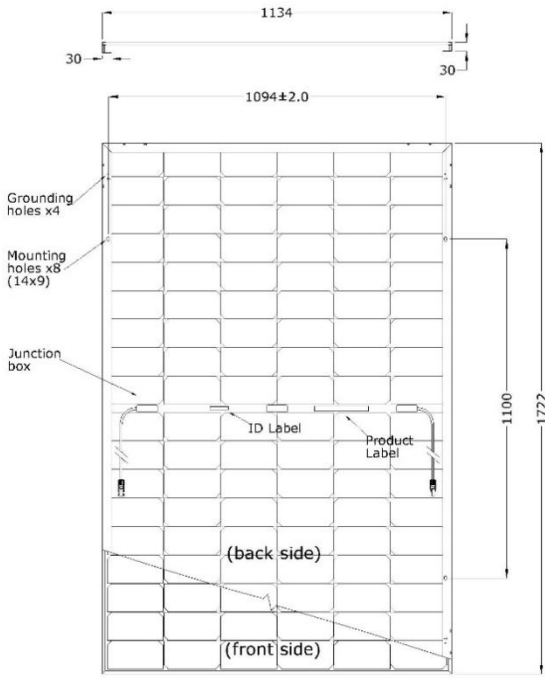
Fig. 5: Mechanical drawing of the FU XXX MV Silk® Nova Duetto (108 half-cut cells) module showing the mounting holes.
