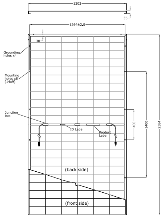
Fig. 10: Mechanical drawing of the FU XXX MV Silk® Nova Premium Max Duetto (132 G12 half-cut cells with) module showing the mounting holes.
