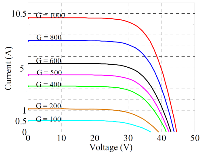
Fig. 1: IV curve at different irradiance
