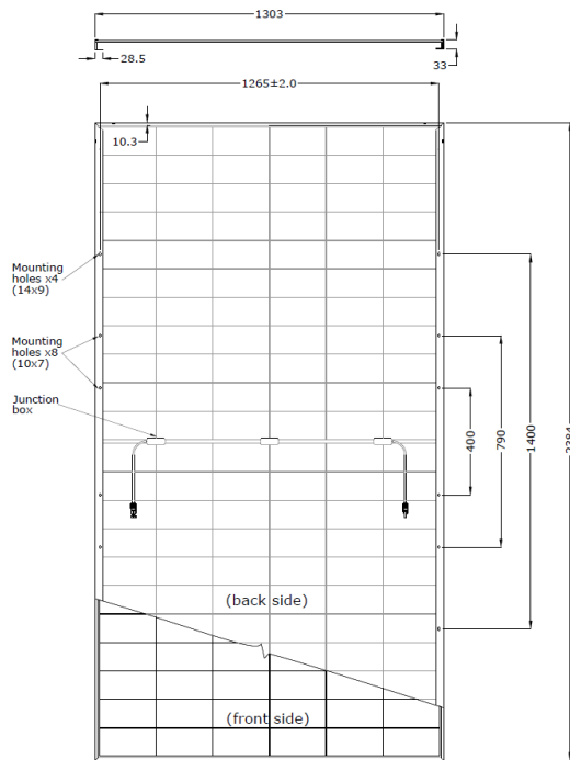
Fig. 11: Mechanical drawing of the FU XXX MV Silk® Nova Premium Max Duetto (132 G12 half-cut cells with frame 33x28.5 and 33x10.3 mm ) module showing the mounting holes.
