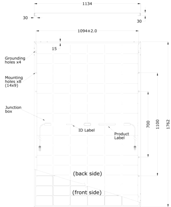
Fig. 8: Mechanical drawing of the FU XXX MV Silk® Nova Duetto (96 half-cut cells) module showing the mounting holes.
