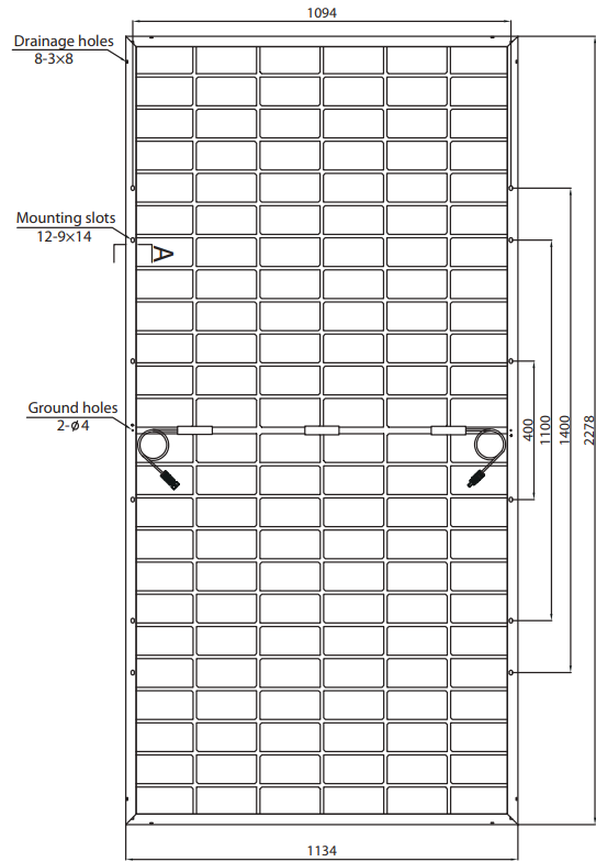
Fig. 6: Mechanical drawing of the FU XXX MV Silk® Nova Duetto (144 half-cut cells with frame 30x30mm) module showing the mounting holes.
