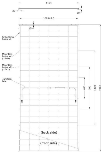
Fig. 9: Mechanical drawing of the FU XXX M/MV Silk® Nova Duetto (132 half-cut cells) module showing the mounting holes.
