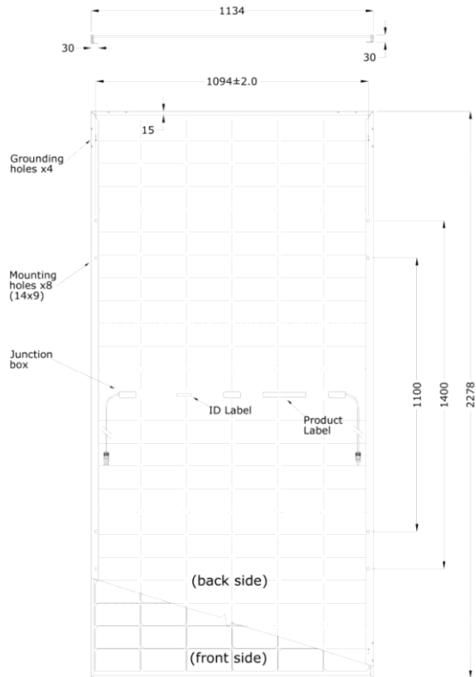
Fig. 7: Mechanical drawing of the FU XXX MV Silk® Nova Duetto (144 M10 half-cut cells with frame 30x30 and 30x15 mm ) module showing the mounting holes.
